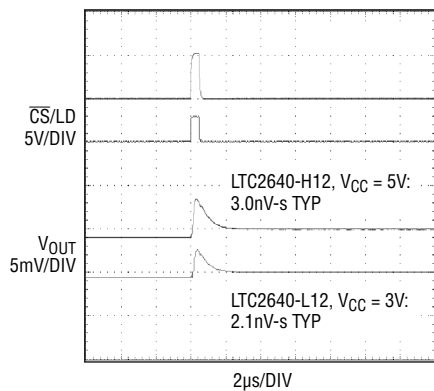
Mid-Scale-Glitch Impulse
