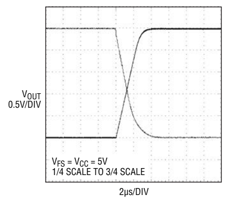
Large-Signal Response
