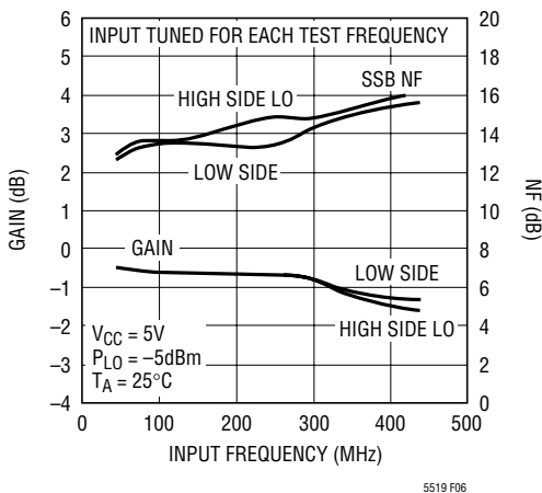
Figure 6. Conversion Gain and Single Sideband Noise Figure vs Tuned IF Input Frequency
