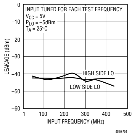
Figure 8. LO to RF Leakage vs Tuned IF Input Frequency
