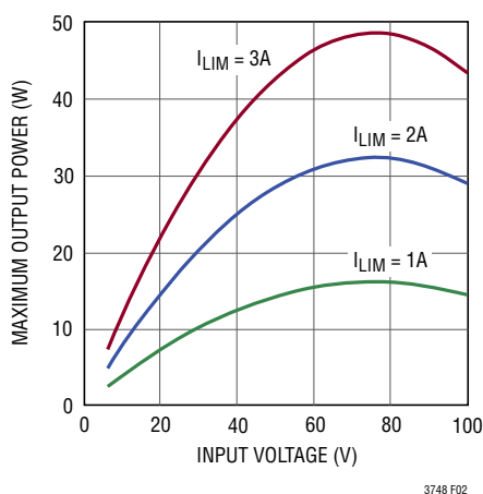
Figure 2. Maximum Output Power at 12V OUT with 150V V_{\text{DS}}(\text{MAX}) and I_{\text{LIM}} = 1\text{A}, 2\text{A}, 3\text{A}
