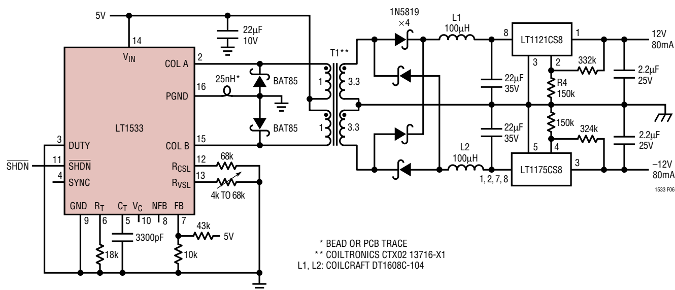
Figure 6. 5V to \pm 12V DC Transformer
