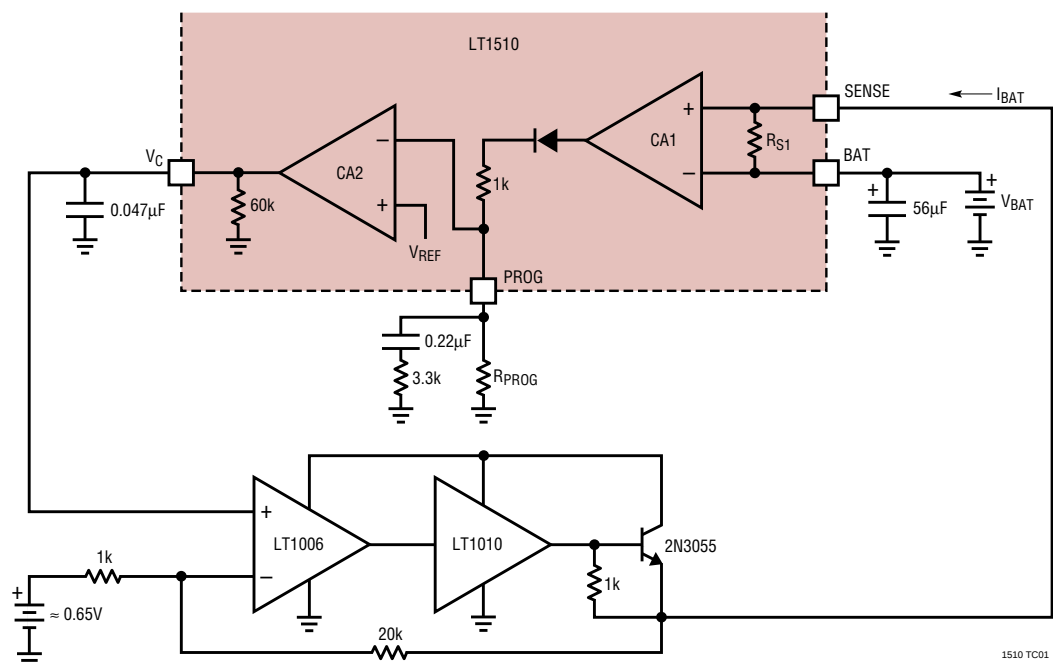
Test Circuit 1
