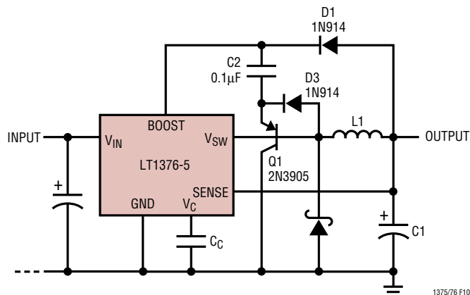
Figure 10. Reducing Minimum Input Voltage
