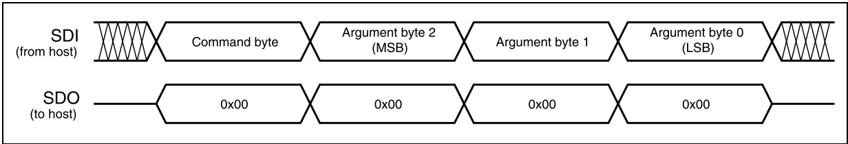
Figure 21. Command with 3-byte argument
