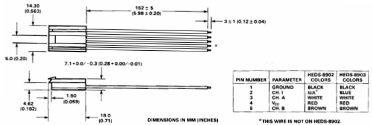
Figure 8. HEDS-8903 Connector.
