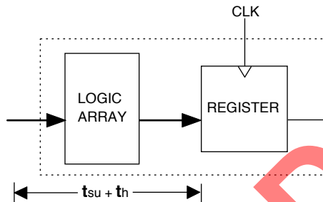
fmax with No Feedback
