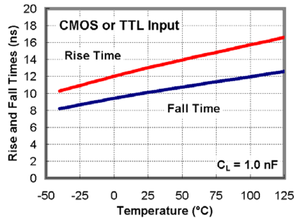
Figure 40. Rise and Fall Times vs. Temperature
