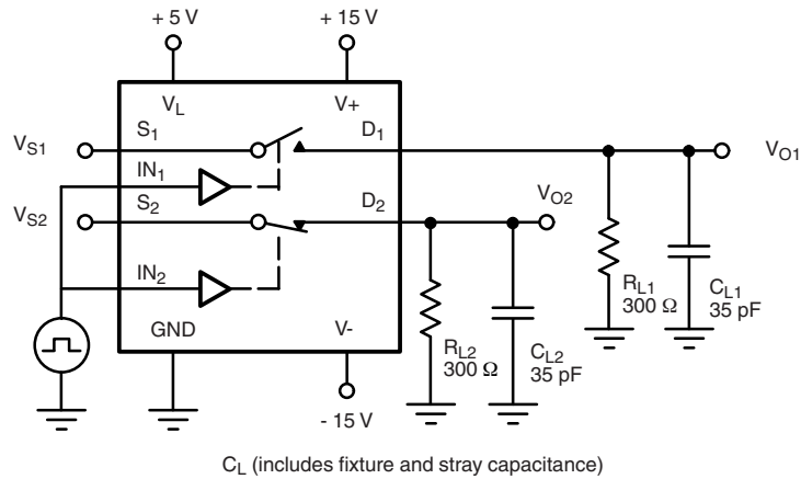
Figure 3. Break-Before-Make (DG413)
