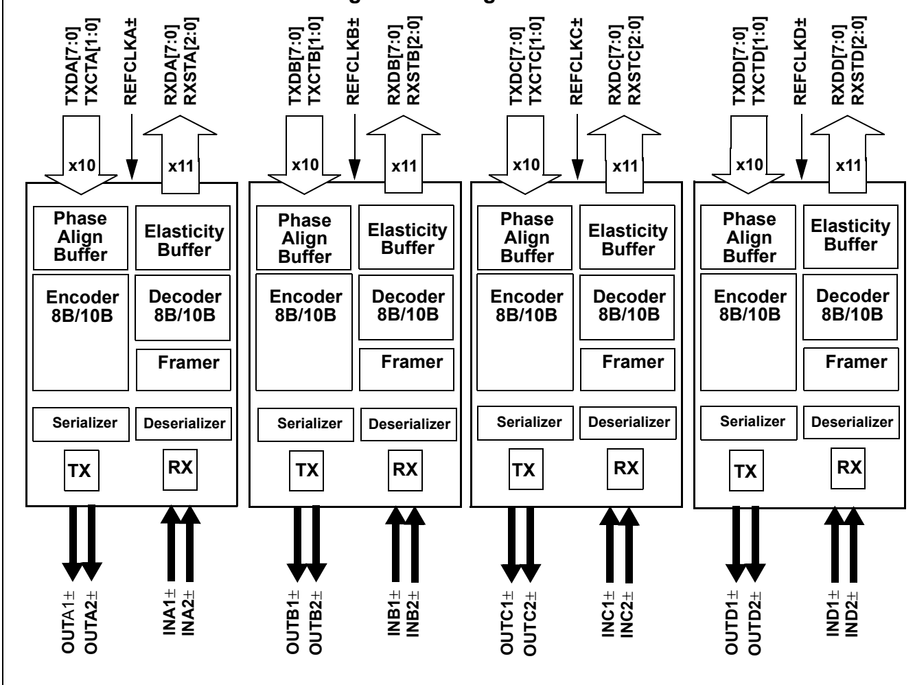
CYV15G0404DXB Transceiver Logic Block Diagram
