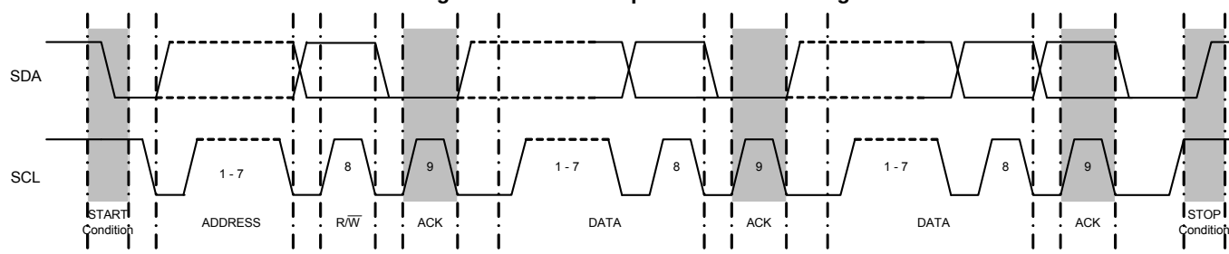
Figure 7-13. I 2 C Complete Transfer Timing
