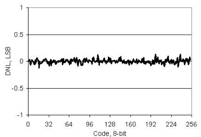
Figure 11-47. VDAC DNL vs. Input Code, 1 V Mode
