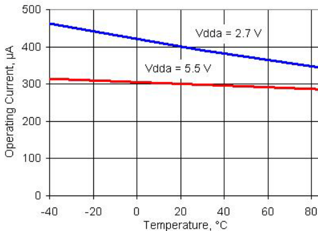
Figure 11-53. VDAC Operating Current vs Temperature, 1 V Mode, Fast Mode
