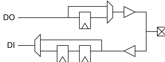
Figure 7-8. I/O Pin Synchronization Routing
