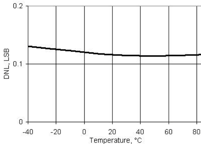
Figure 11-51. VDAC DNL vs Temperature, 1 V Mode
