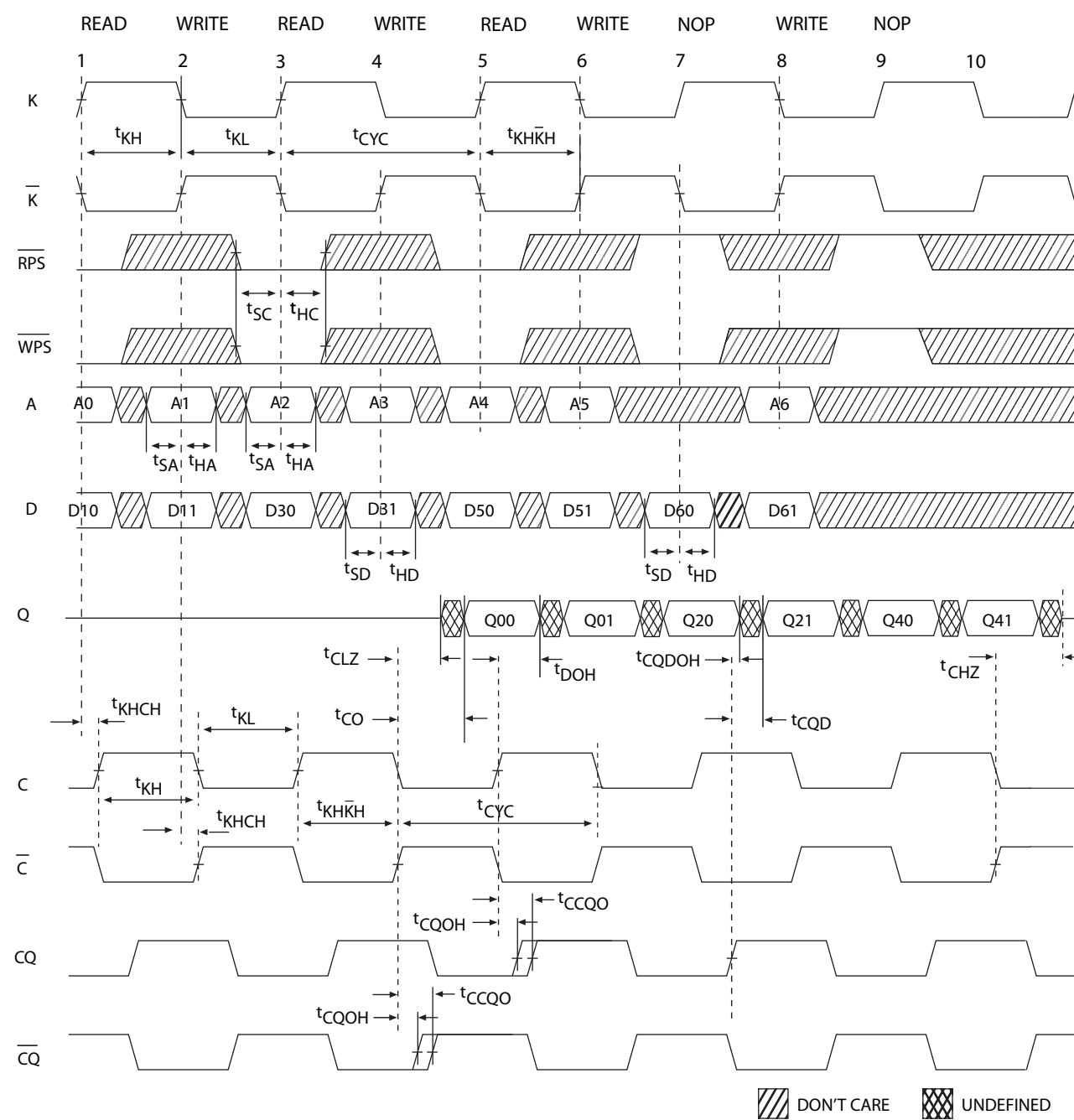
Figure 5. Read/Write/Deselect Sequence [26, 27, 28]
