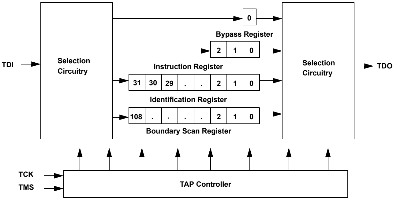
TAP Controller Block Diagram
