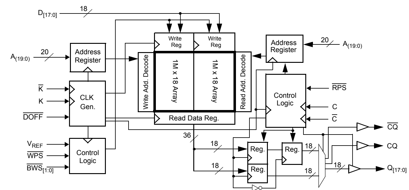
Logic Block Diagram – CY7C1412AV18
