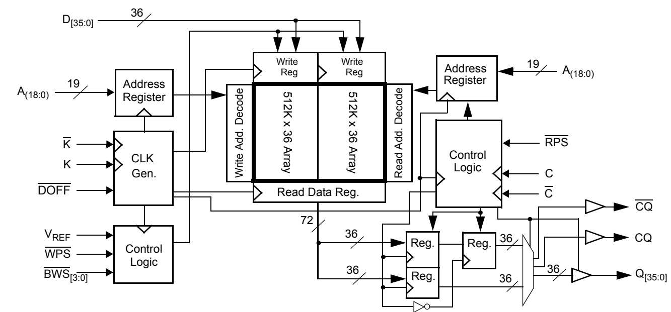
Logic Block Diagram – CY7C1414AV18
