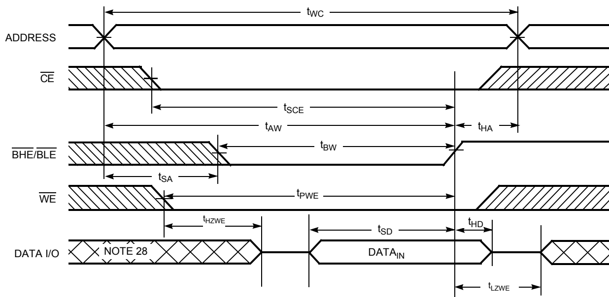
Figure 10. Write Cycle No. 4 ( \overline{BHE/BL} controlled, \overline{OE} LOW) [26]
