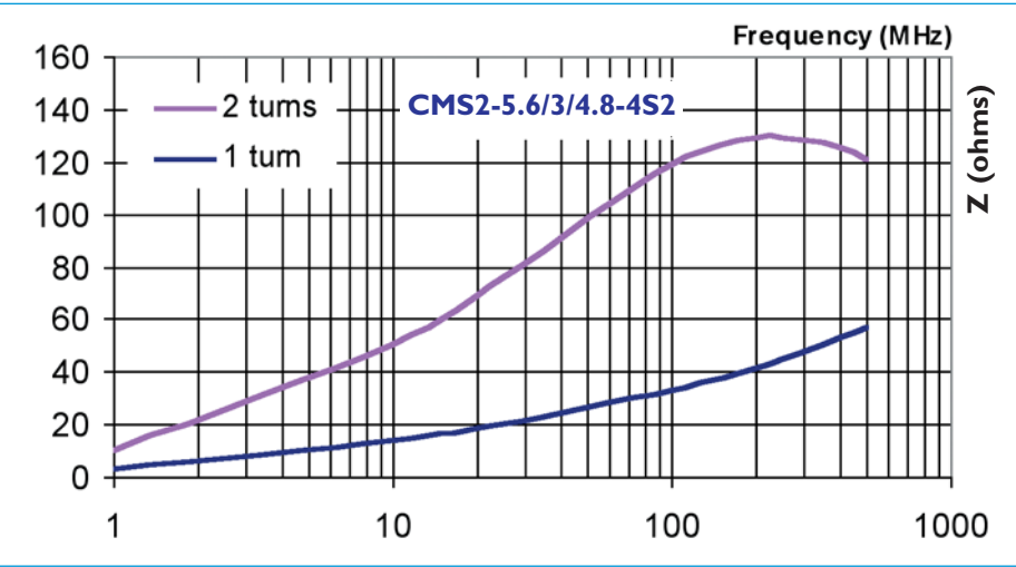
5.2.7 TYPICAL IMPEDANCE CURVES
