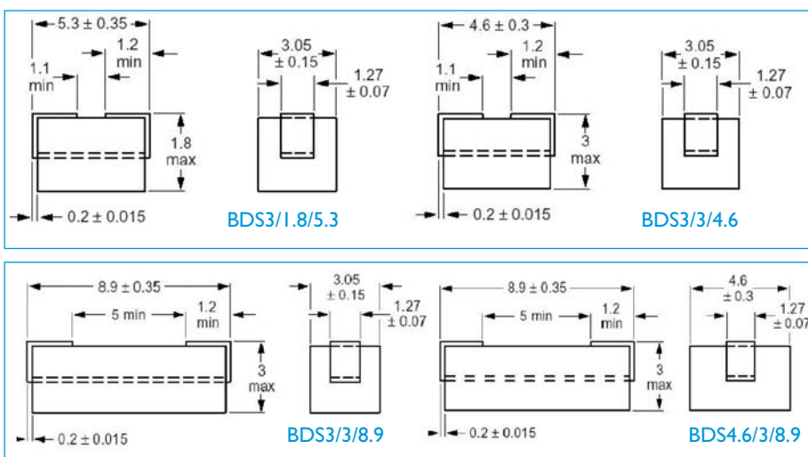
Figure 4. Chip bead dimensions (in millimeters)
