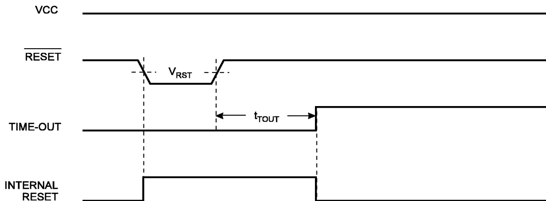
Figure 27. External Reset During Operation
