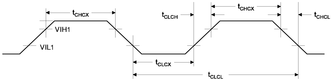
Figure 38. Waveforms
