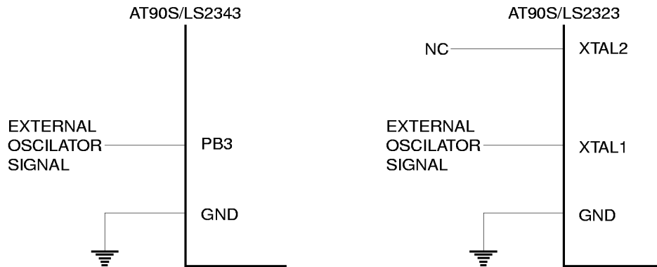
Figure 4. External Clock Drive Configuration
