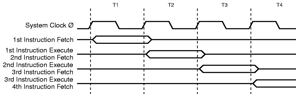
Figure 21. The Parallel Instruction Fetches and Instruction Executions
