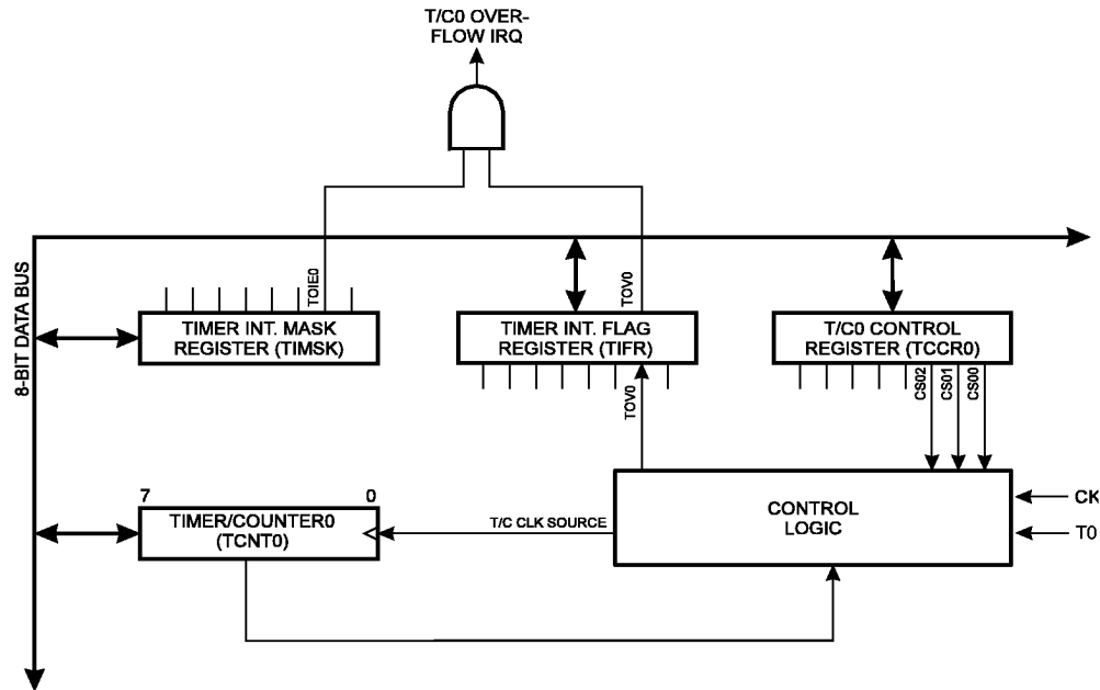
Figure 30. Timer/Counter 0 Block Diagram
