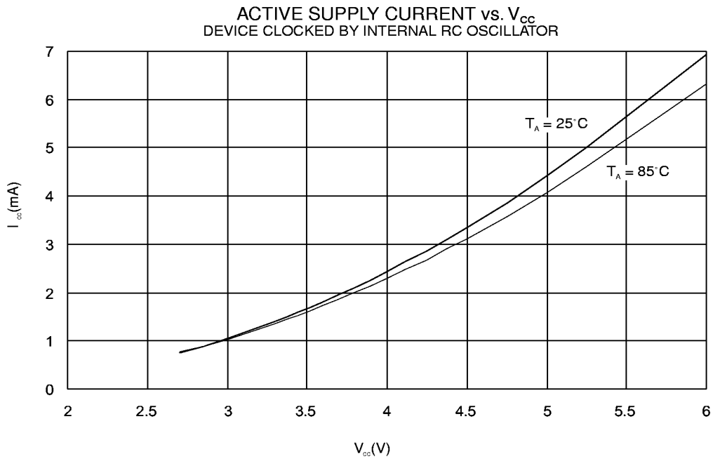
Figure 41. Active Supply Current vs. V_{CC}
