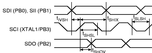
Figure 34. High-voltage Serial Programming Timing
