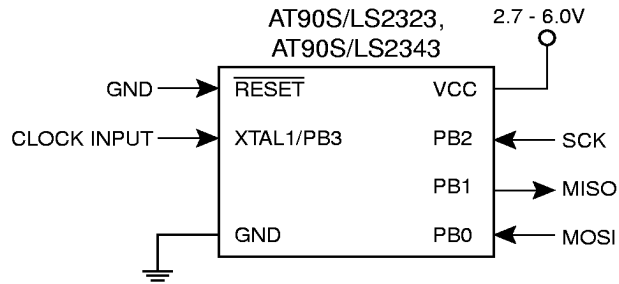
Figure 35. Low-Voltage Serial Programming and Verify
