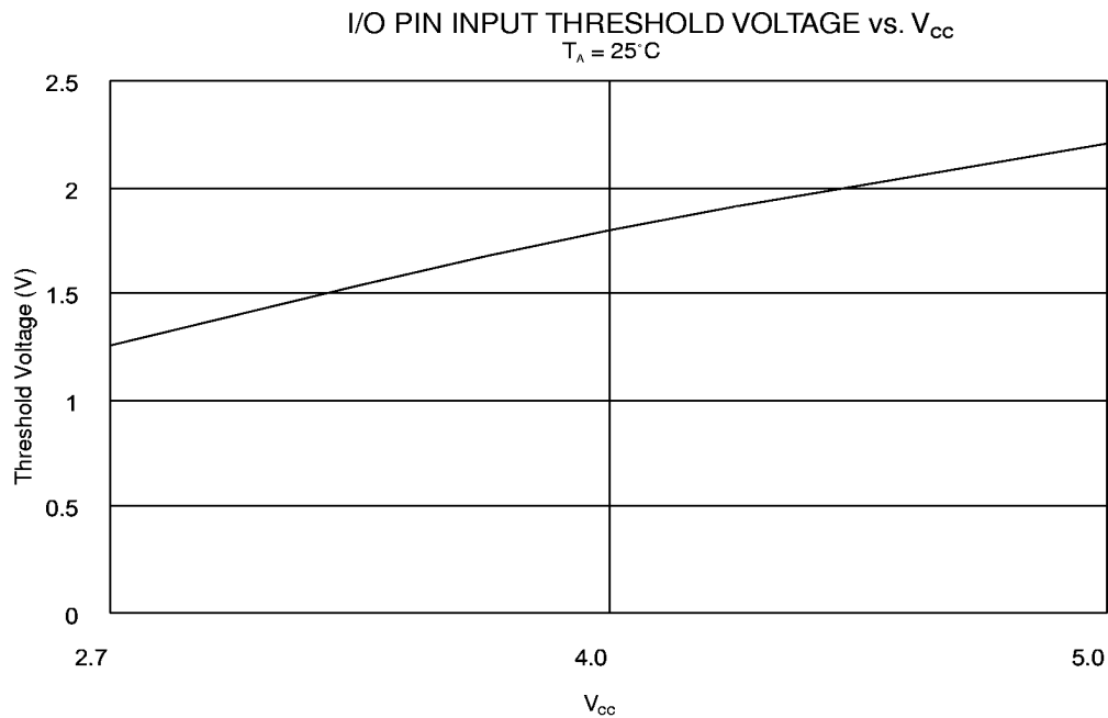
Figure 54. I/O Pin Input Threshold Voltage vs. V_{CC}
