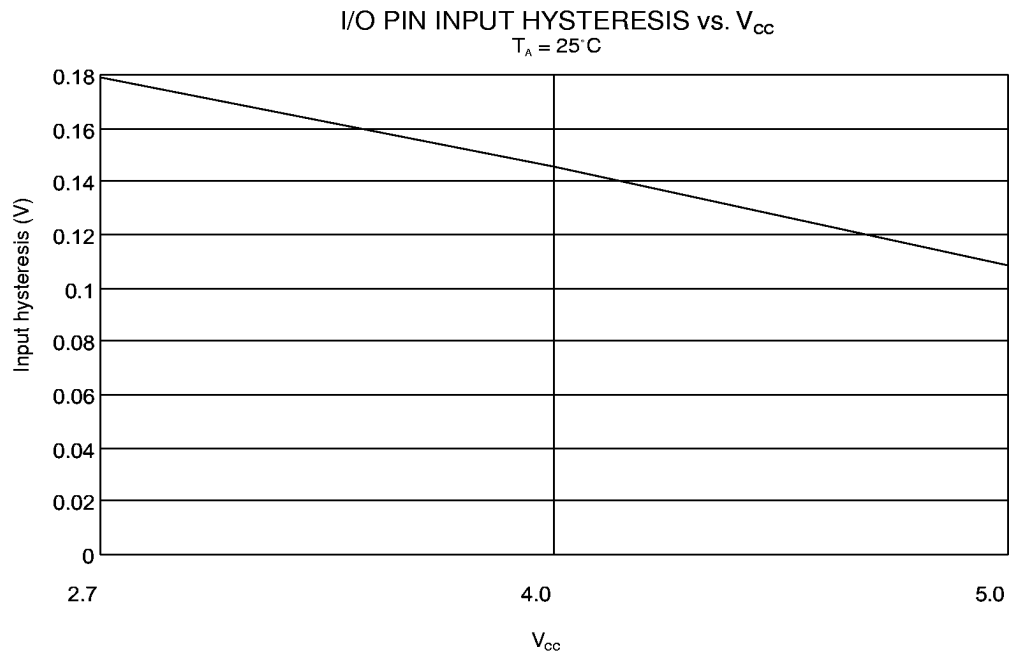
Figure 55. I/O Pin Input Hysteresis vs. V_{CC}
