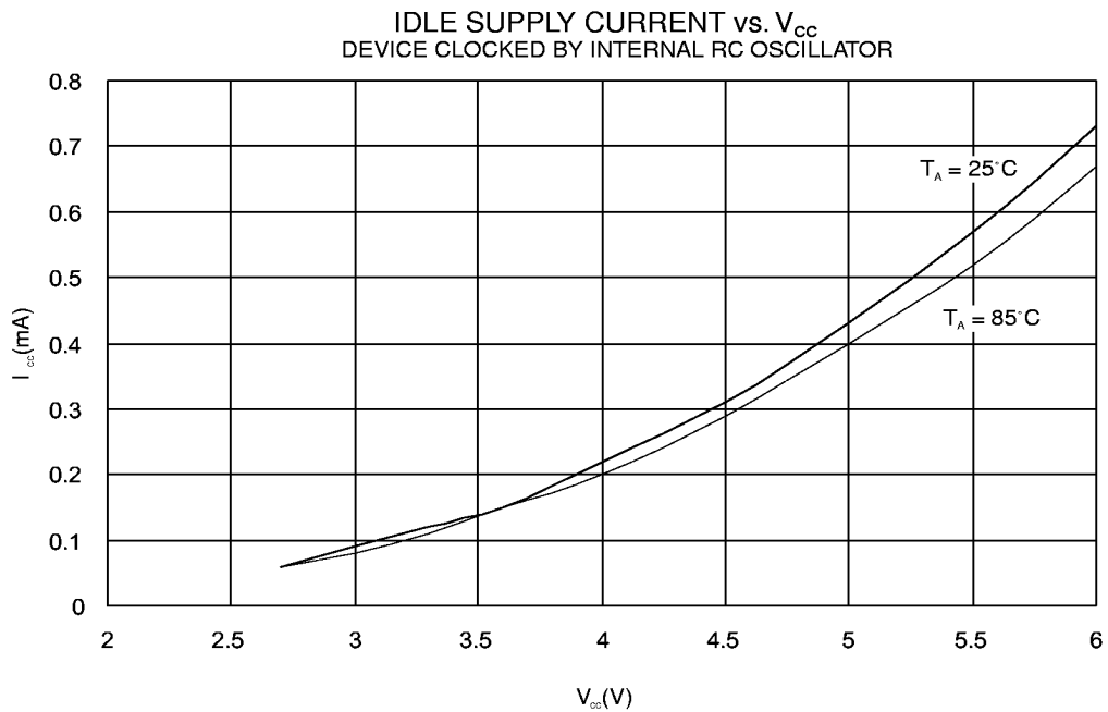
Figure 44. Idle Supply Current vs. V_{CC}
