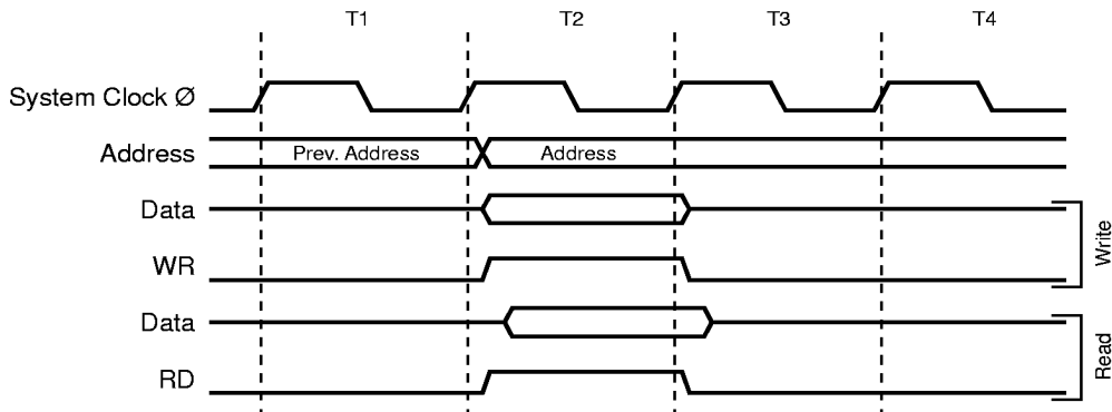
Figure 23. On-chip Data SRAM Access Cycles
