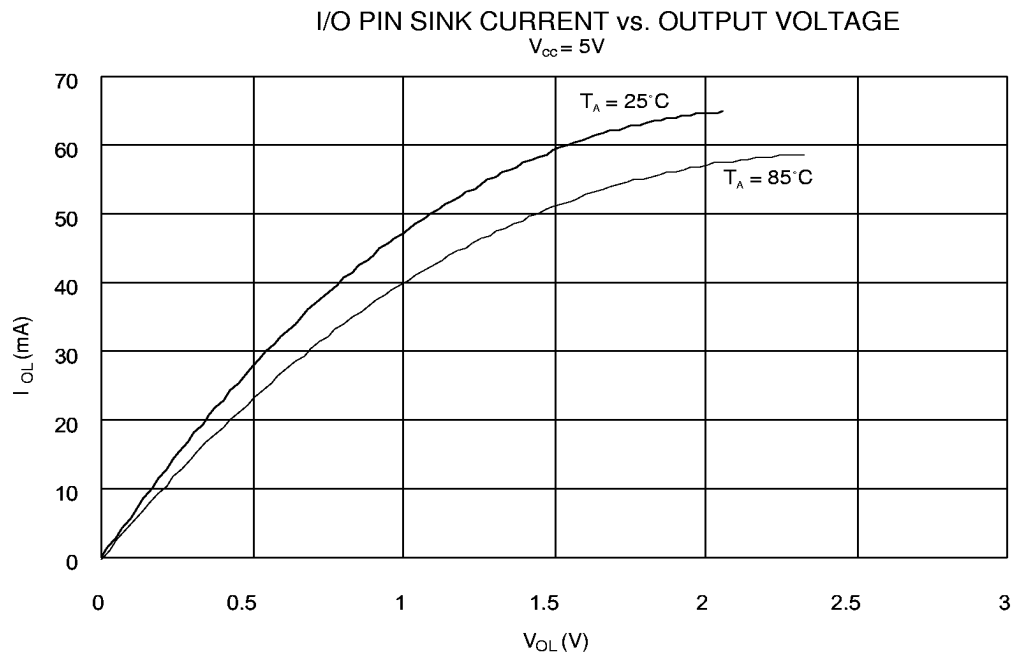
Figure 50. I/O Pin Sink Current vs. Output Voltage
