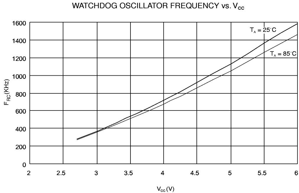
Figure 47. Watchdog Oscillator Frequency vs. V_{CC}
