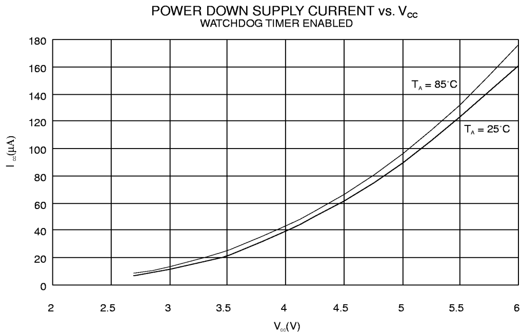
Figure 46. Power Down Supply Current vs. V_{CC}
