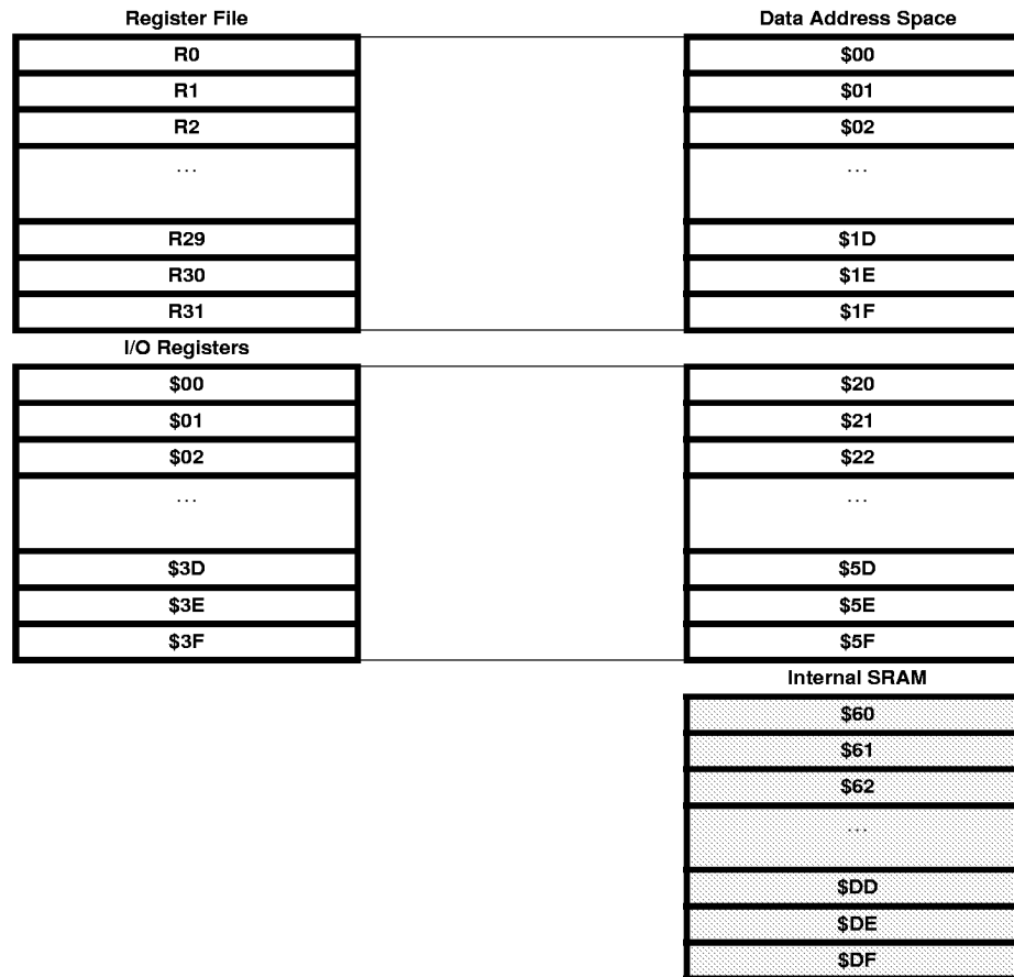
Figure 9. SRAM Organization
