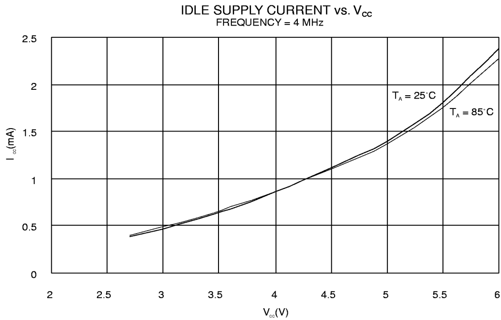
Figure 43. Idle Supply Current vs. V_{CC}
