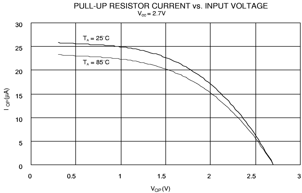
Figure 49. Pull-up Resistor Current vs. Input Voltage
