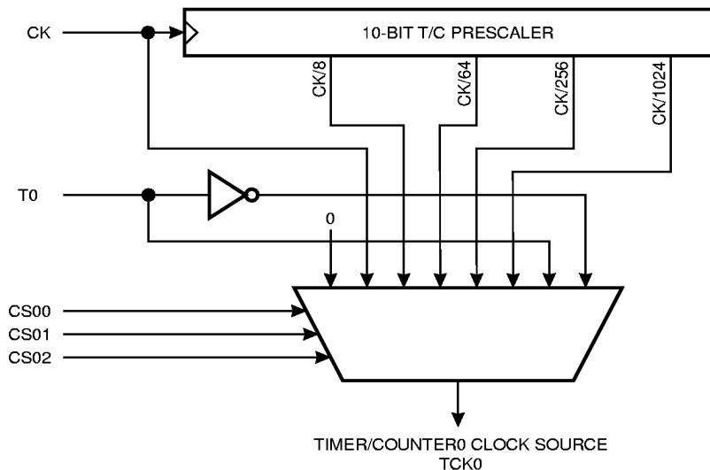
Figure 29. Timer/Counter0 Prescaler
