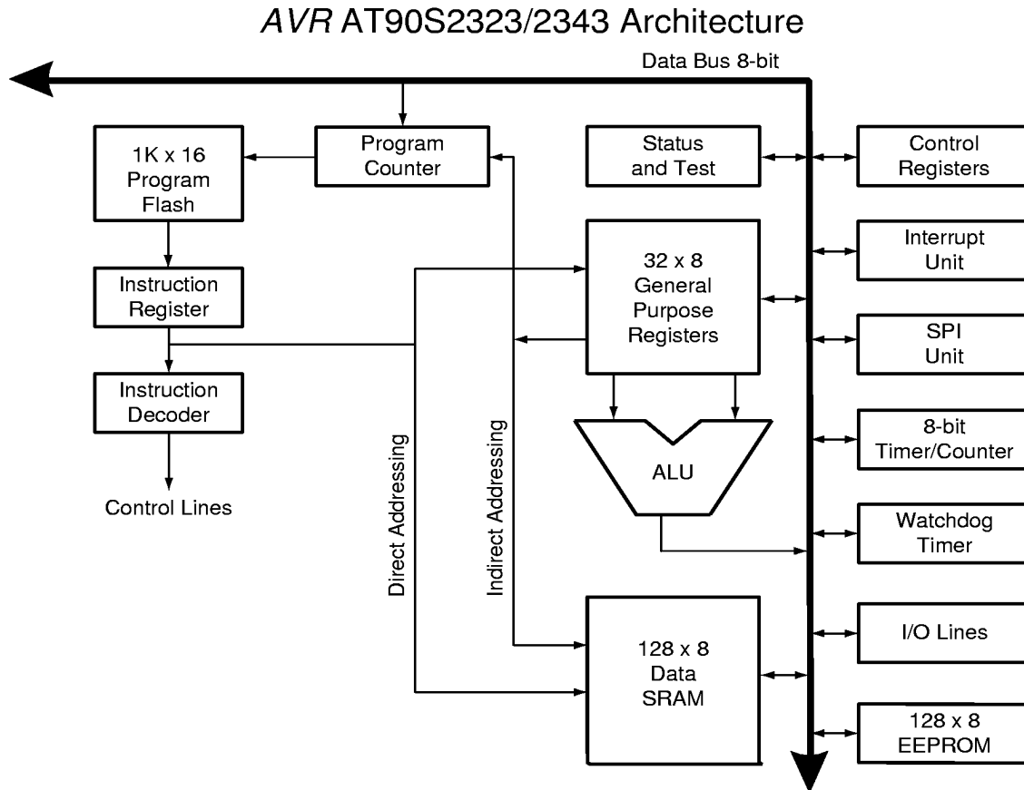
Figure 5. The AT90S2323/2343 AVR RISC Architecture
