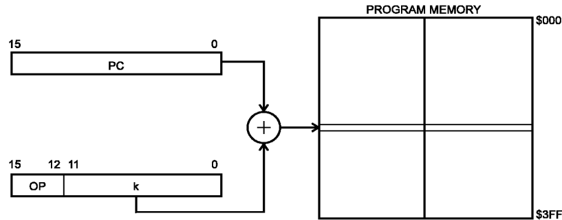
Figure 20. Relative Program Memory Addressing
