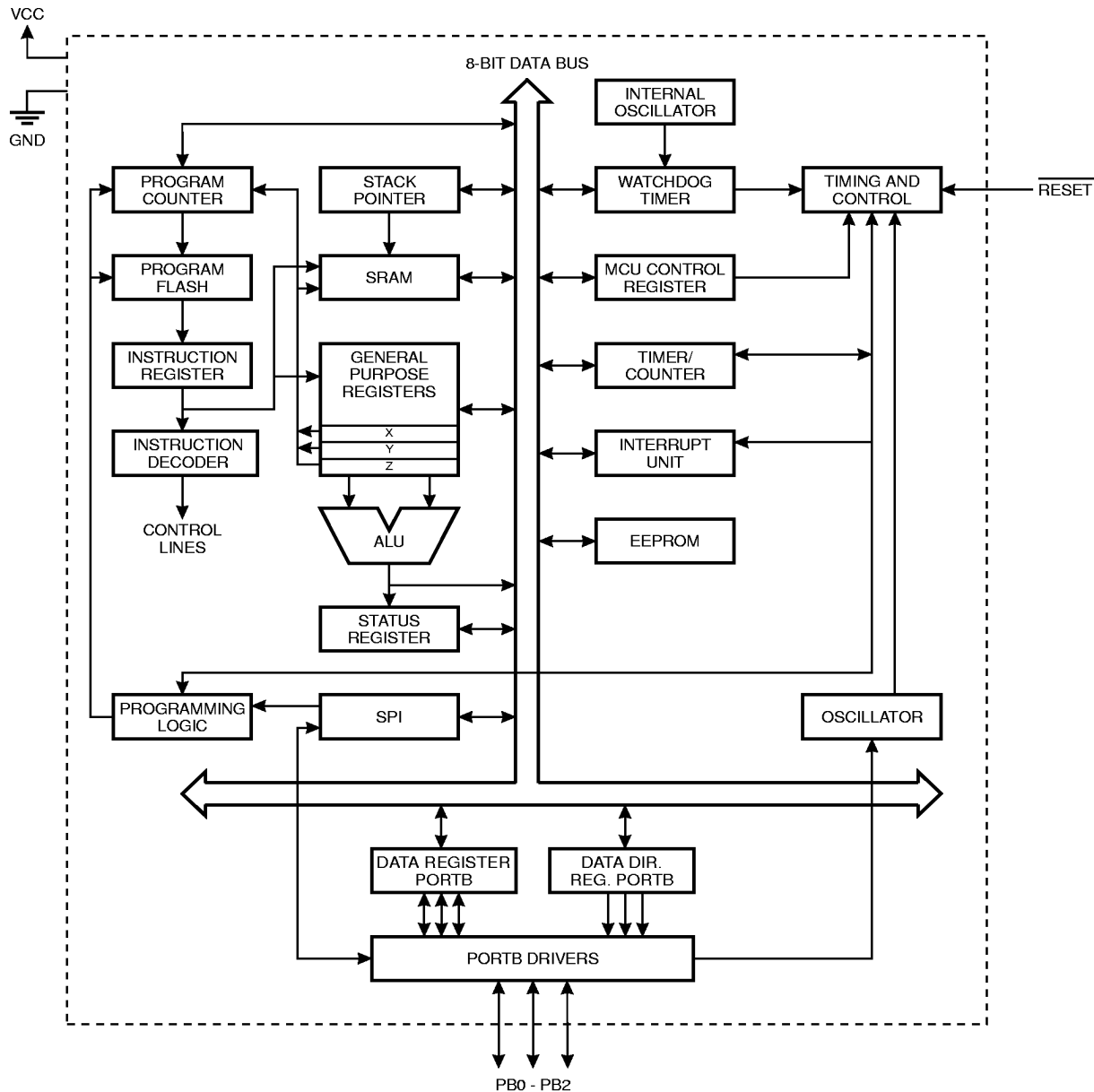
Figure 2. The AT90S/LS2323 Block Diagram
