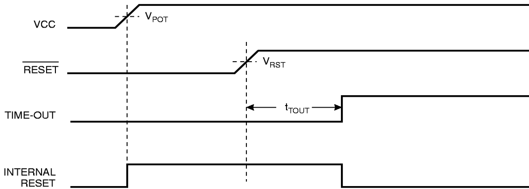
Figure 26. MCU Start-Up, \overline{\text{RESET}} Controlled Externally
