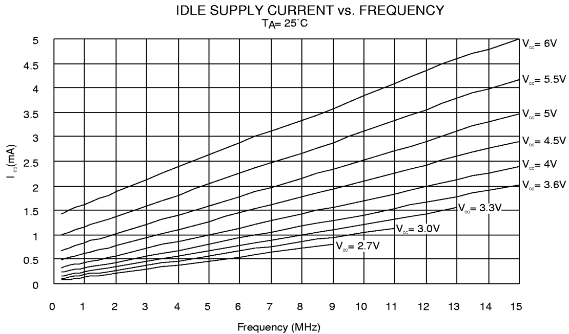
Figure 42. Idle Supply Current vs. Frequency
