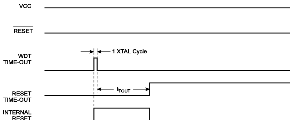
Figure 28. Watchdog Reset During Operation
