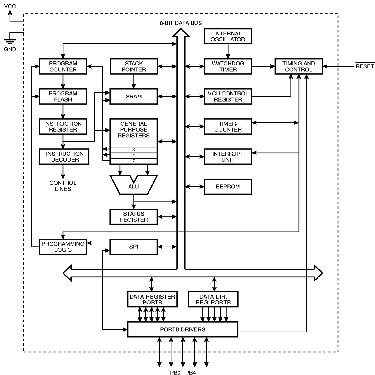
Figure 1. The AT90S/LS2343 Block Diagram
