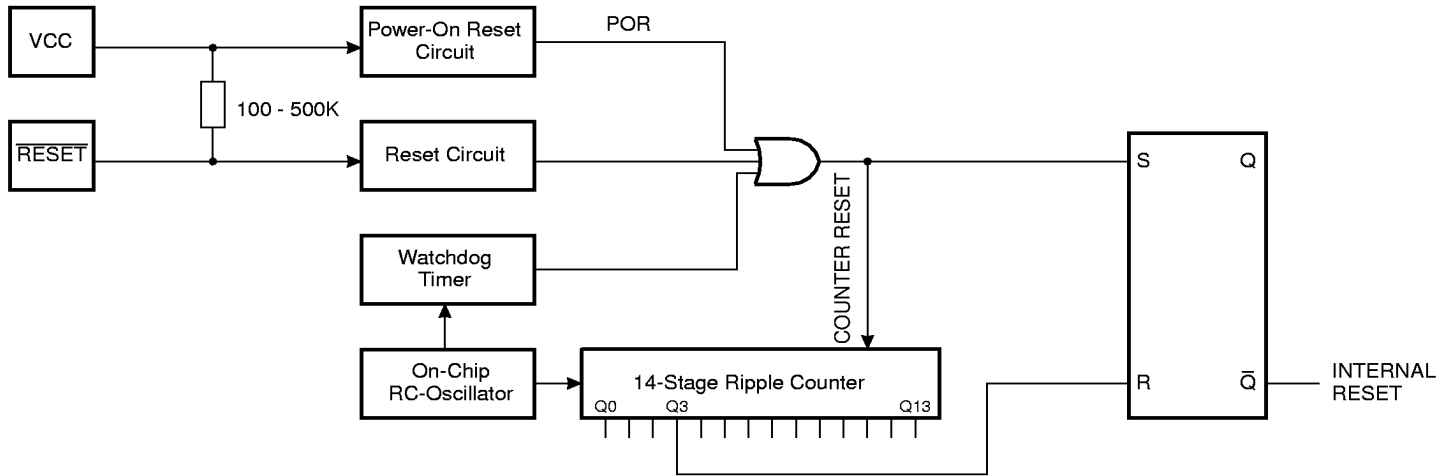
Figure 24. Reset Logic
