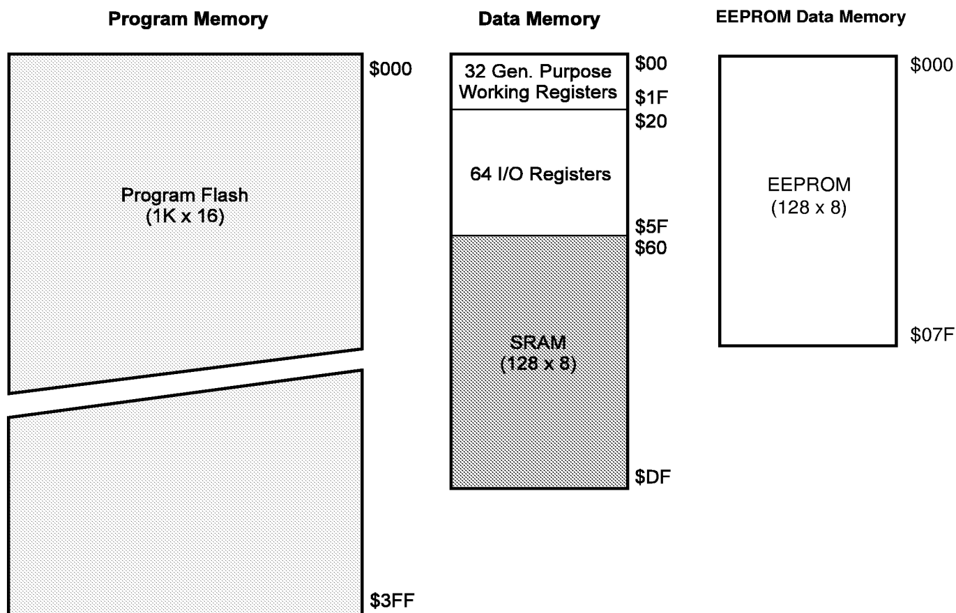
Figure 6. Memory Maps
