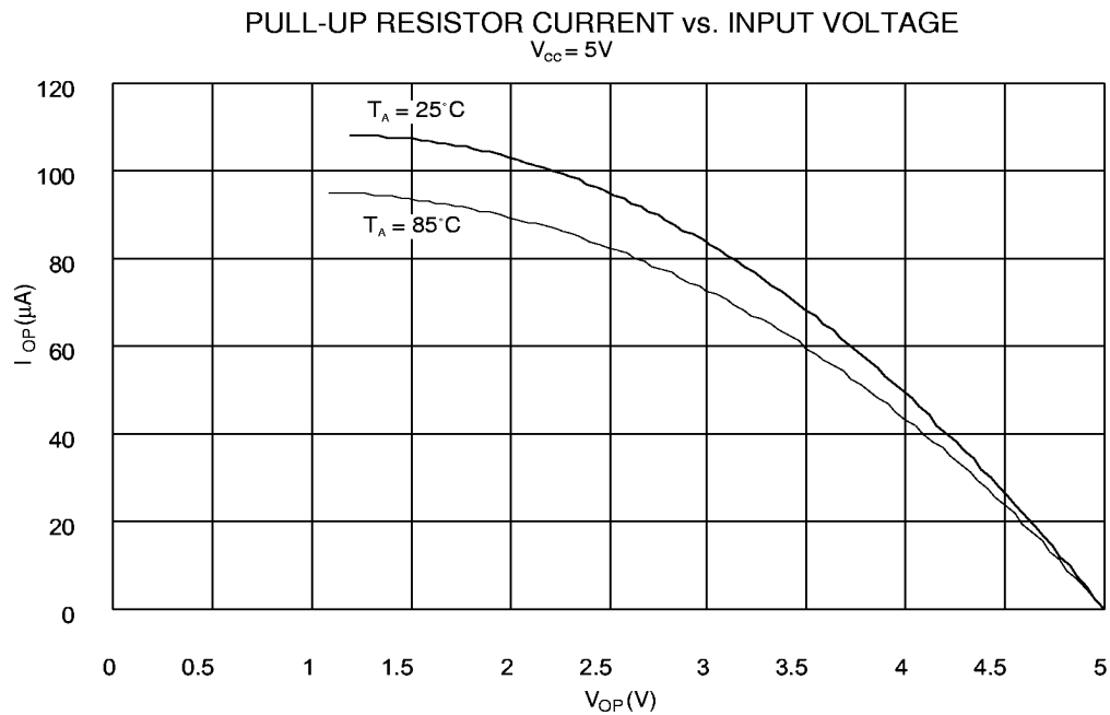
Figure 48. Pull-up Resistor Current vs. Input Voltage
