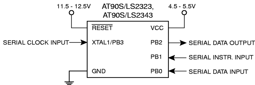
Figure 32. High-voltage Serial Programming
