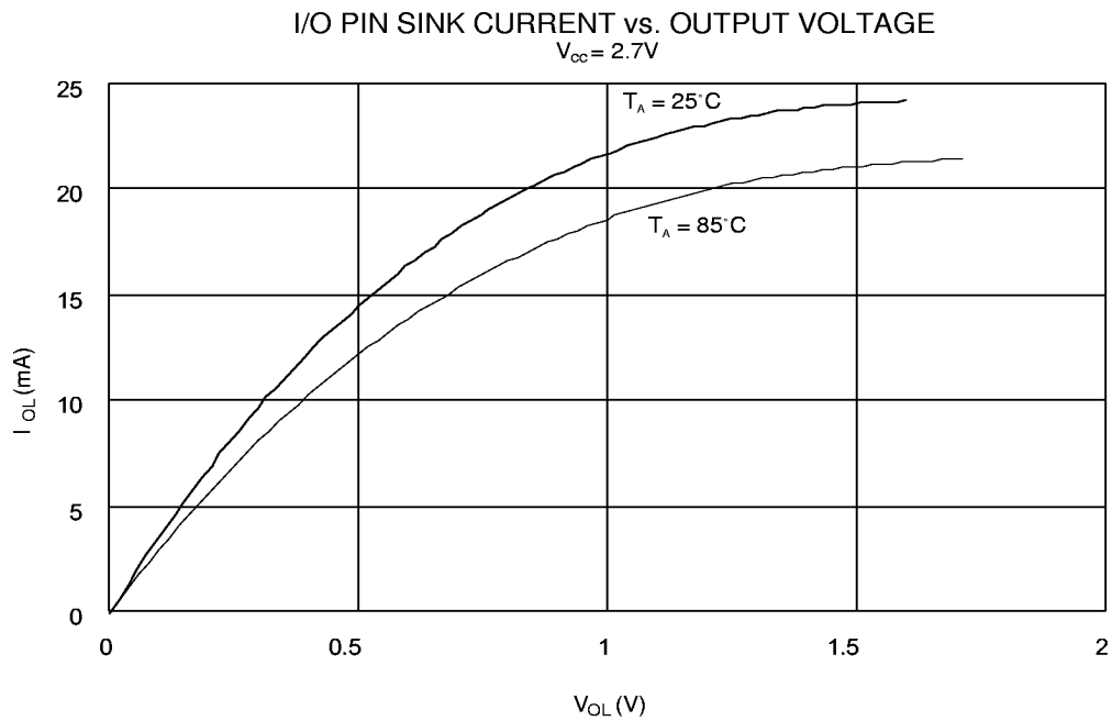
Figure 52. I/O Pin Sink Current vs. Output Voltage
