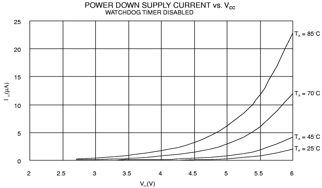
Figure 45. Power Down Supply Current vs. V_{CC}
