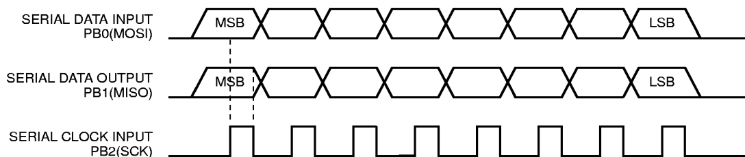
Figure 36. Low-voltage Serial Downloading Waveforms
