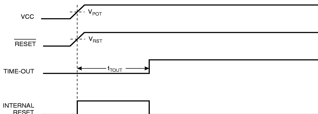
Figure 25. MCU Start-Up, \overline{RESET} Tied to V_{CC} .
