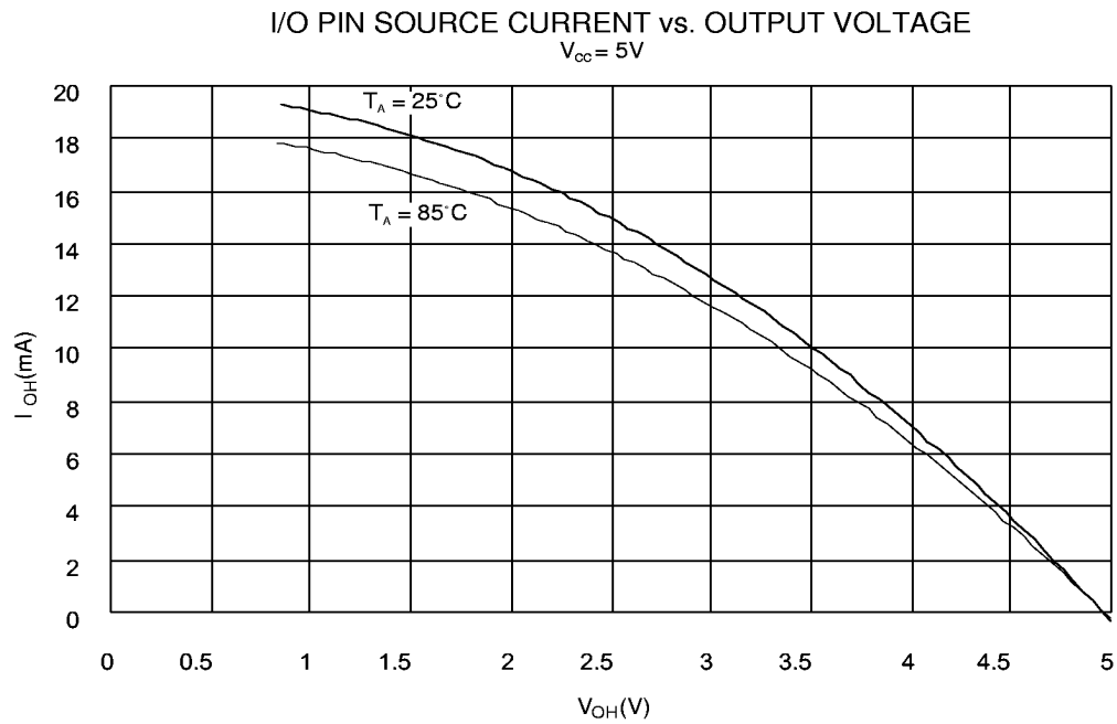
Figure 51. I/O Pin Source Current vs. Output Voltage
