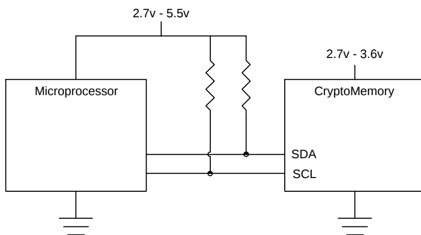
Figure 4-1. Connection Diagram
