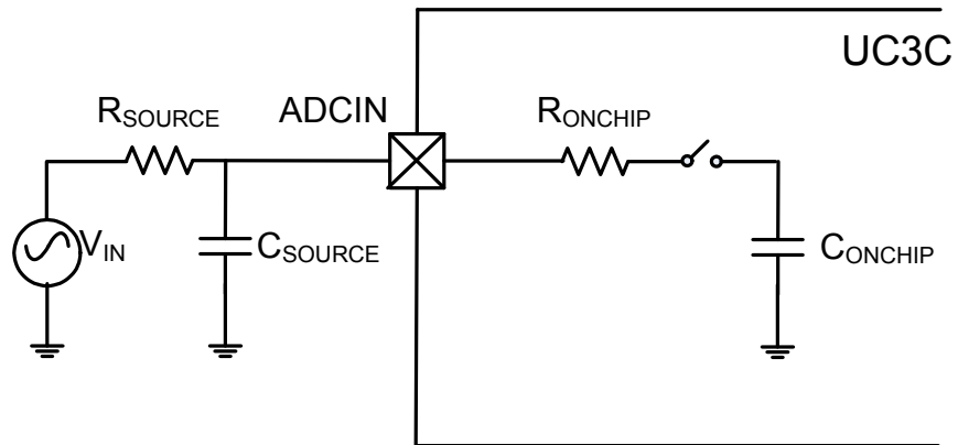
Figure 7-3. ADC input
