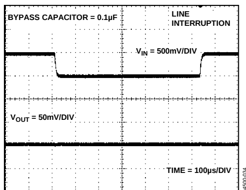
Figure 23. ADR431 Line Transient Response, 0.1 μF Bypass Capacitor
