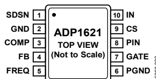
Figure 4. Pin Configuration
