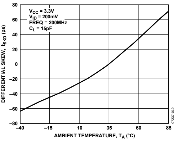
Figure 19. Differential Skew, t_{SKD} vs. Ambient Temperature, T_A
