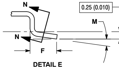
DETAIL E
