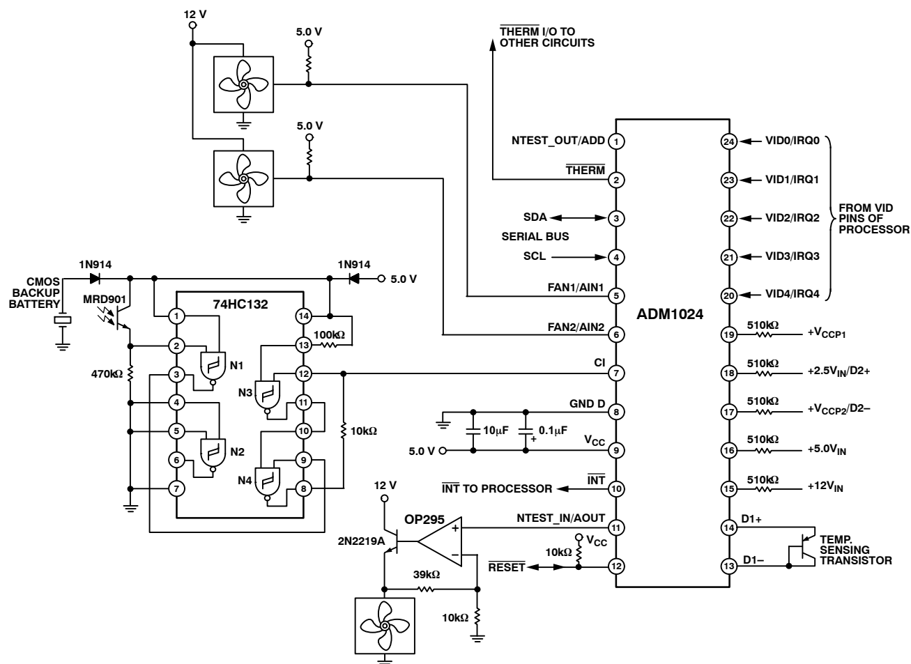
Figure 37. Application Circuit
