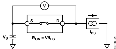
Figure 19. On Resistance
