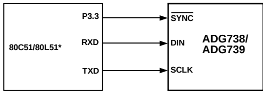
Figure 28. 8051 Interface to ADG738/ADG739
