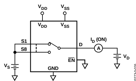
Figure 24. I_D (ON)
