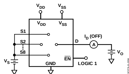
Figure 23. I_D (OFF)
