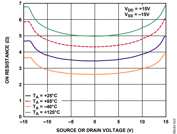
Figure 11. On Resistance as a Function of V_D ( V_S ) for Different Temperatures, \pm 15 V Dual Supply
