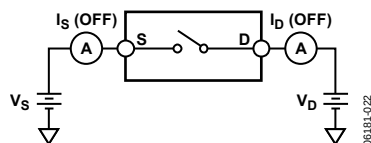
Figure 26. Off Leakage
