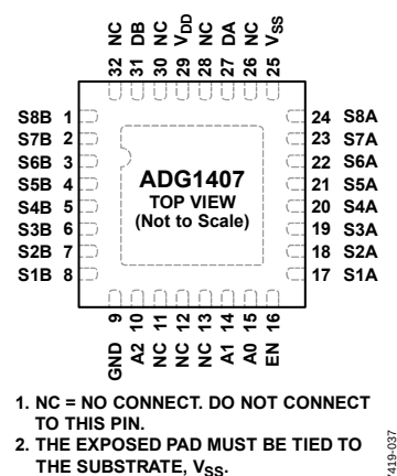
Figure 6. ADG1407 LFCSP Pin Configuration
