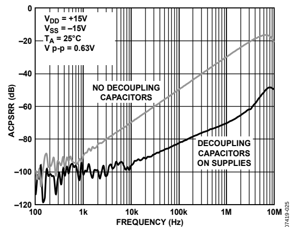
Figure 26. ACPSSR vs. Frequency
