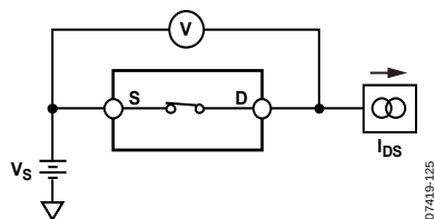
Figure 27. On Resistance
