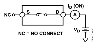
Figure 29. On Leakage
