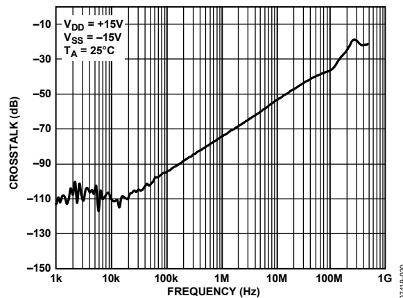
Figure 21. ADG1406 Crosstalk vs. Frequency
