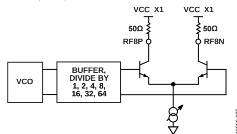
Figure 41. Output Stage
