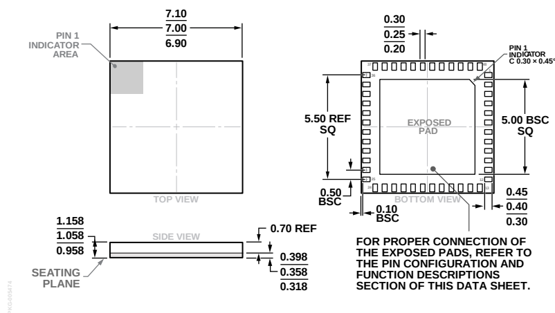
Figure 45. 48-Terminal Land Grid Array [LGA] (CC-48-4) Dimensions shown in millimeters
