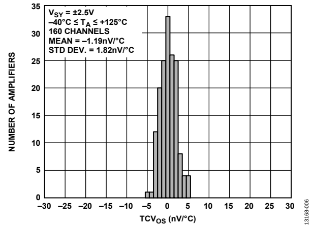
Figure 9. Input Offset Voltage Drift Distribution, V_{SY} = \pm 2.5\text{ V}
