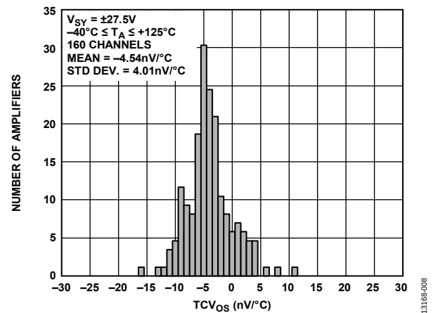
Figure 11. Input Offset Voltage Drift Distribution, V_{SY} = \pm 27.5\text{ V}
