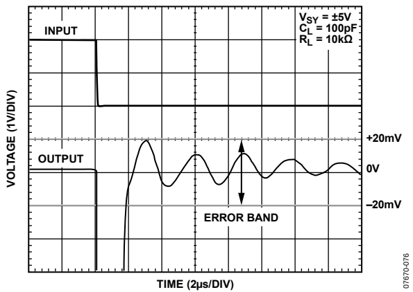
Figure 43. Negative Settling Time to 0.1%
