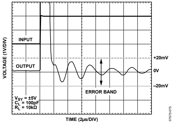
Figure 42. Positive Settling Time to 0.1%
