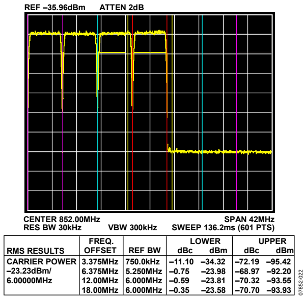
Figure 45. 4-Channel QAM ACLR, f_{OUT} = 840 MHz, Temperature = 25°C, Sum Scale = 20, Full-Scale Current = 25 mA, Span = 42 MHz, Channel 4
