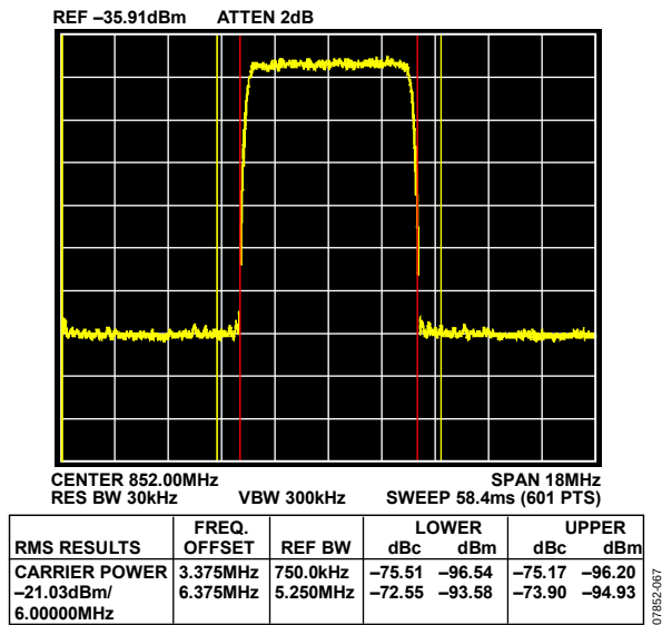
Figure 44. Zoomed 2-Channel QAM ACLR, f_{OUT} = 840 MHz, Sum Scale = 32, Full-Scale Current = 25 mA, Span = 18 MHz, Channel 2
