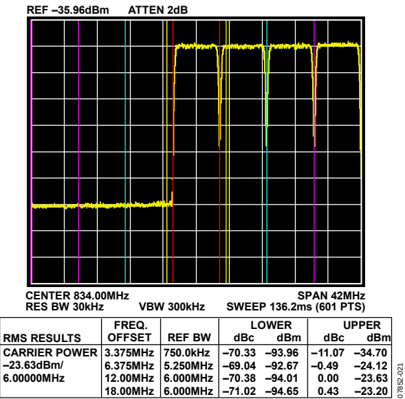
Figure 43. 4-Channel QAM ACLR, f_{OUT} = 840 MHz, Temperature = 25°C, Sum Scale = 20, Full-Scale Current = 25 mA, Span = 42 MHz, Channel 1
