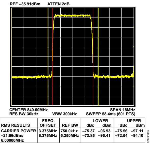
Figure 42. Zoomed 2-Channel QAM ACLR, f_{OUT} = 840 MHz, Sum Scale = 32, Full-Scale Current = 25 mA, Span = 18 MHz, Channel 1
