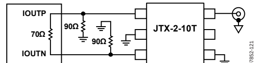
Figure 110. Recommended Transformer Output Stage for Single-Tone/Multitone Measurements
