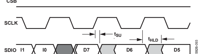
Figure 77. Timing Diagram for SPI Register Read
