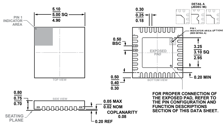
Figure 91. 32-Lead Lead Frame Chip Scale Package [LF CSP] 5 mm × 5 mm and 0.75 mm Package Height (CP-32-7)
