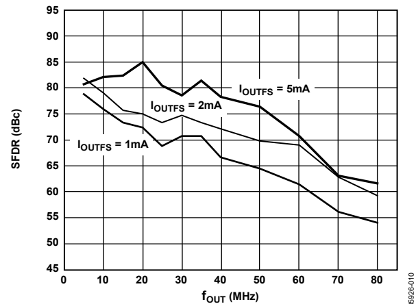
Figure 12. SFDR vs. f_{OUT} and I_{OUTFS} @ 175 MSPS
