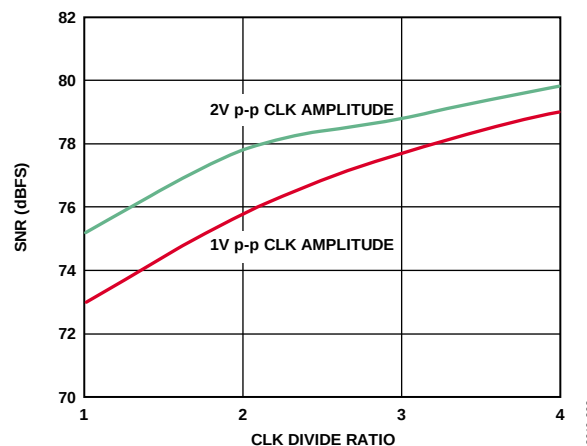
Figure 92. SNR vs. CLK Divide Ratio for f_{IN} = 141 MHz and a Sample Rate of 105 MSPS
