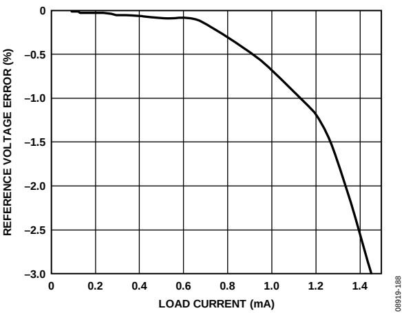
Figure 84. Reference Voltage Error vs. Load Current
