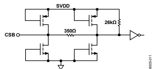
Figure 60. Equivalent CSB Input Circuit
