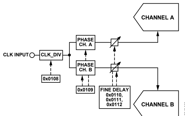
Figure 68. Clock Divider Phase and Delay Controls
