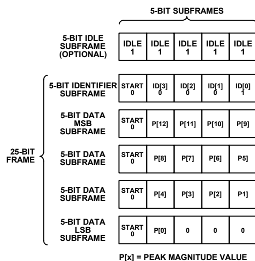
Figure 104. SPORT over JESD204B Signal Monitor Frame Data
