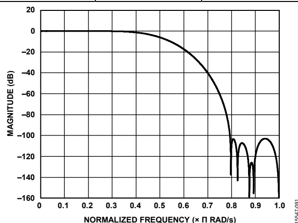
Figure 96. HB2 Filter Response
