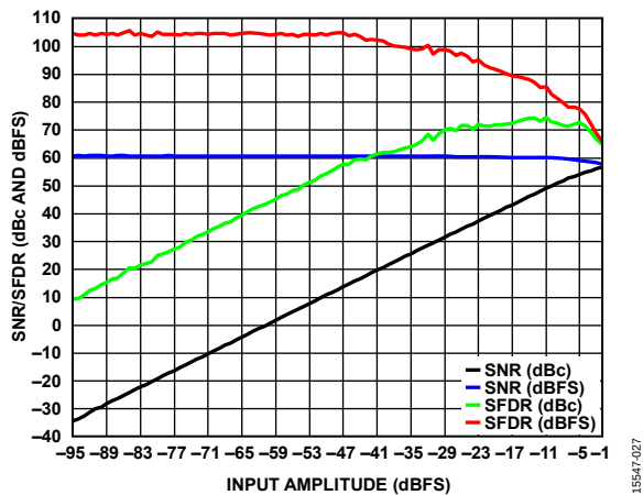
Figure 31. SNR/SFDR vs. Input Amplitude ( A_{IN} ), f_{IN} = 950 MHz
