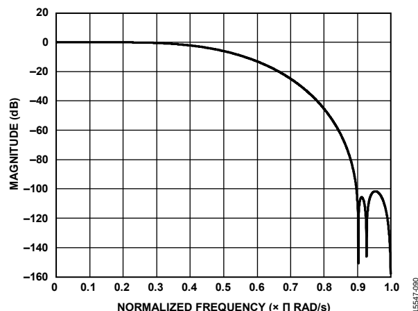
Figure 95. HB3 Filter Response
