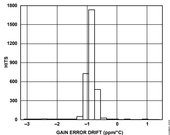
Figure 28. Gain Error Drift Distribution
