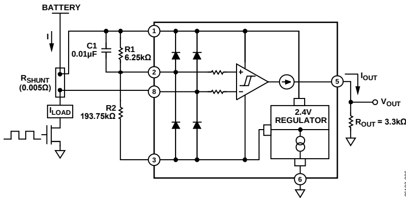
Figure 30. Typical Application
