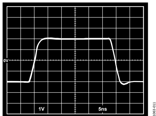
Figure 9. Large Step Response, G = -1 (See Figure 35)
