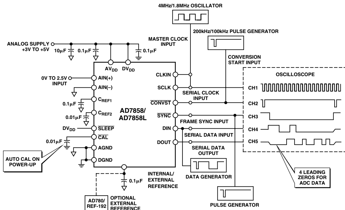
Figure 10. Typical Circuit
