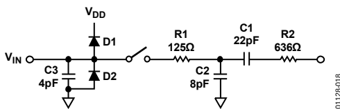
Figure 18. Equivalent Analog Input Circuit
