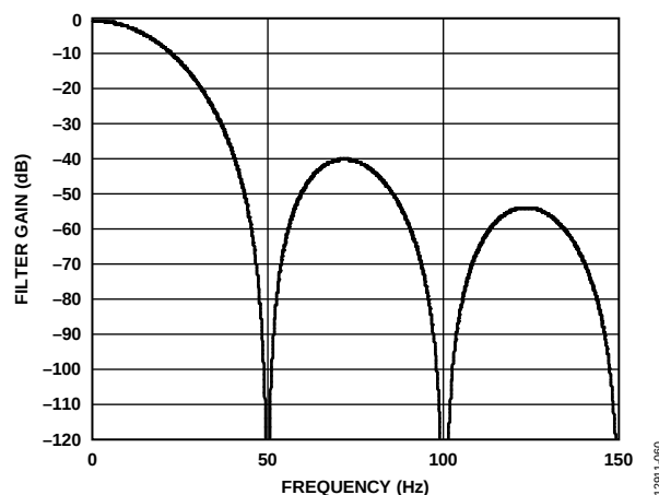
Figure 56. Sinc3 Filter Response
