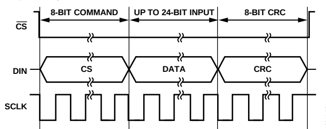
Figure 70. SPI Write Transaction with CRC
