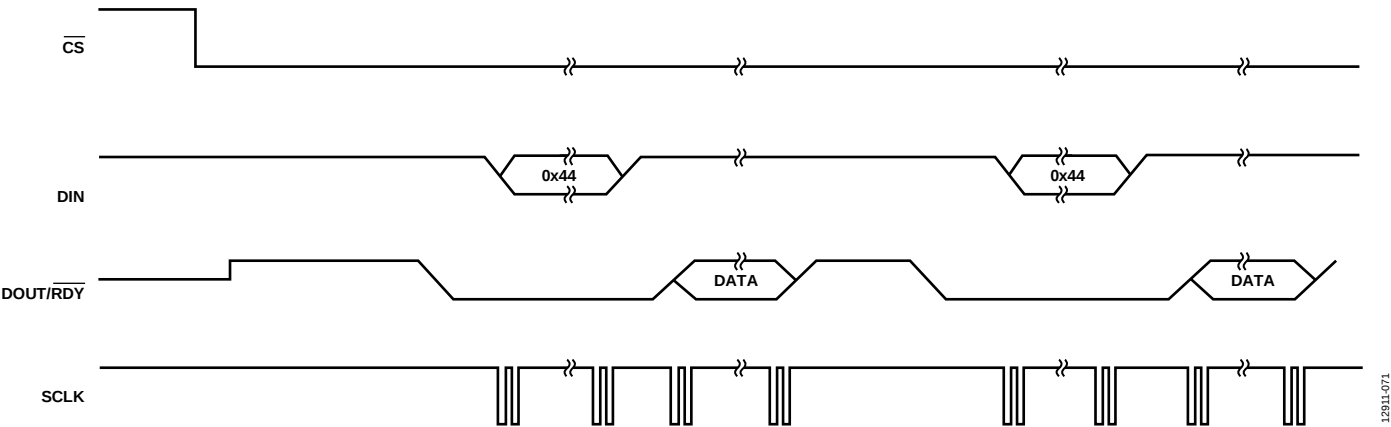
Figure 67. Continuous Conversion Mode
