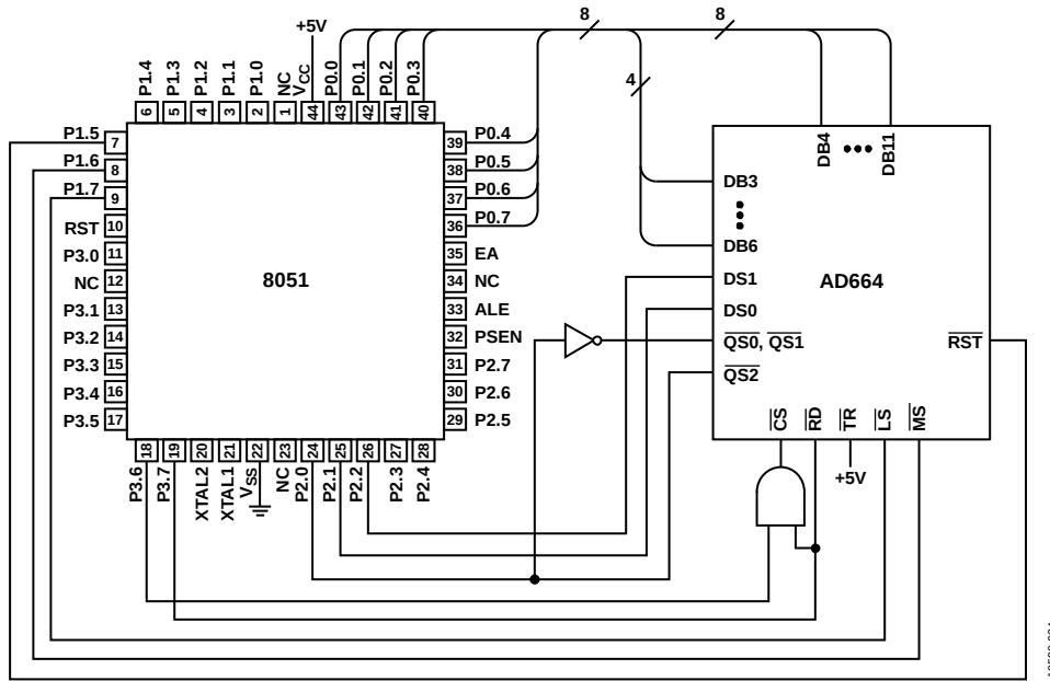
Figure 36. AD664 to 8051 Interface
