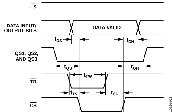
Figure 25. Fully Transparent Mode
