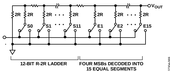
Figure 71. DAC Ladder Structure
