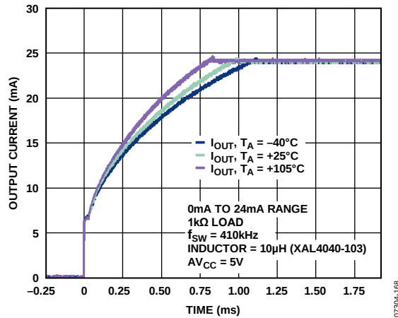
Figure 50. Output Current Settling with DC-to-DC Converter vs. Time and Temperature (See Figure 79)
