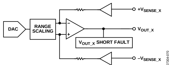
Figure 72. Voltage Output
