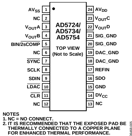
Figure 5. Pin Configuration
