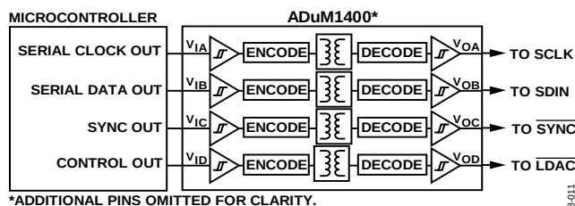
Figure 45. Isolated Interface
