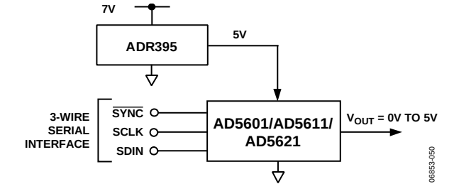
Figure 51. ADR395 as Power Supply to the AD5601/AD5611/AD5621
