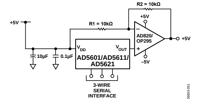
Figure 52. Bipolar Operation with the AD5601/AD5611/AD5621
