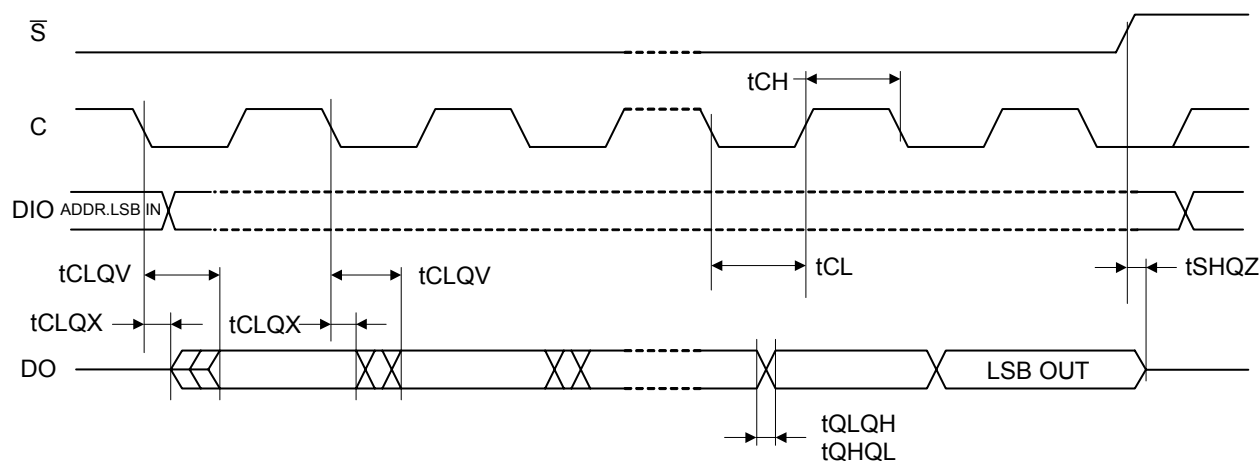
Figure 26. Output Timing
