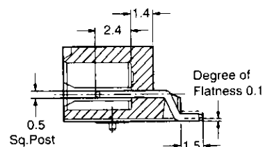
Section X-X
