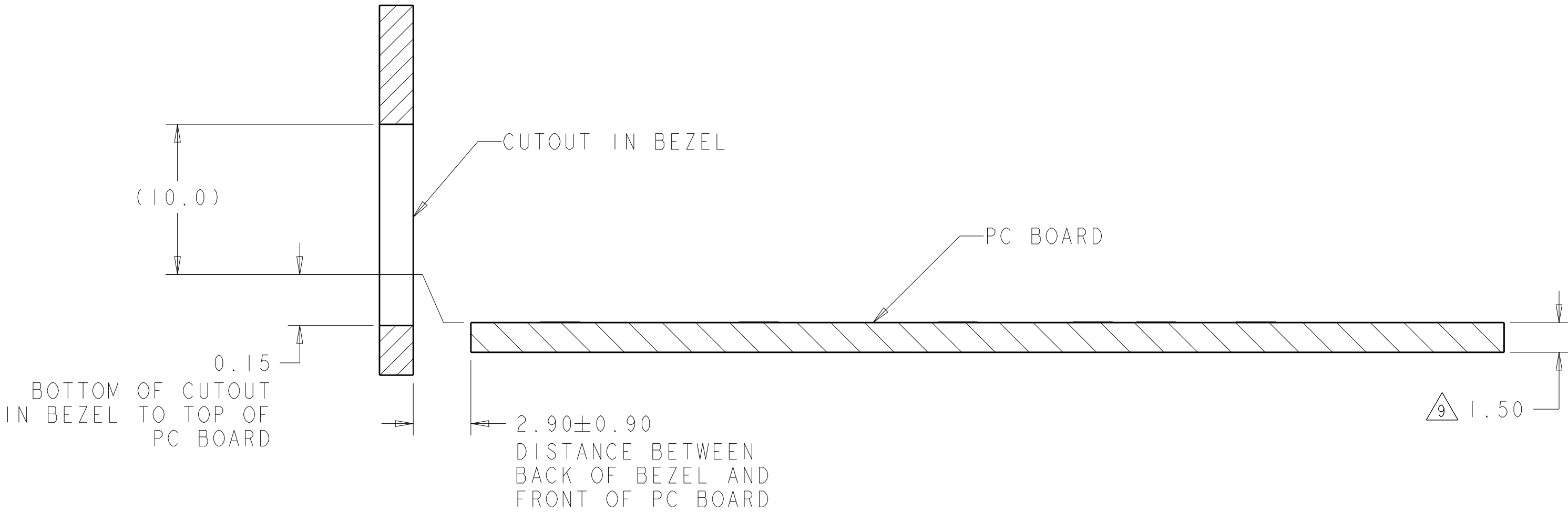
SECTION F-F RECOMMENDED BEZEL CONFIGURATION
