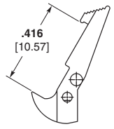
Short Latch Part No. 102312-1 (See Figure 2)
