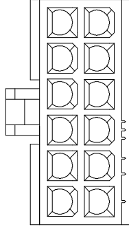
12 POS
